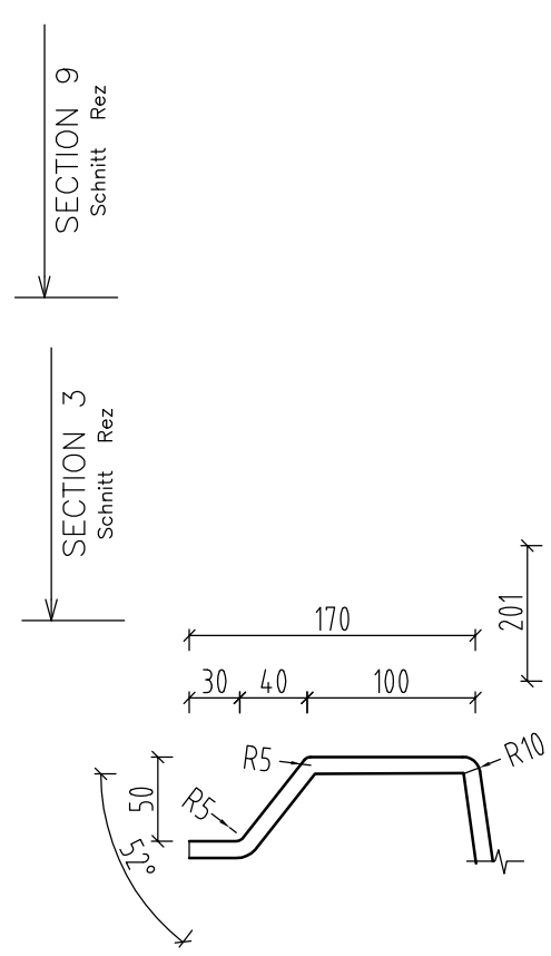
BORDER DETAIL BORD DETAIL DETAIL LEMU SCALE 1:10 MASSTABBE MIERKA
